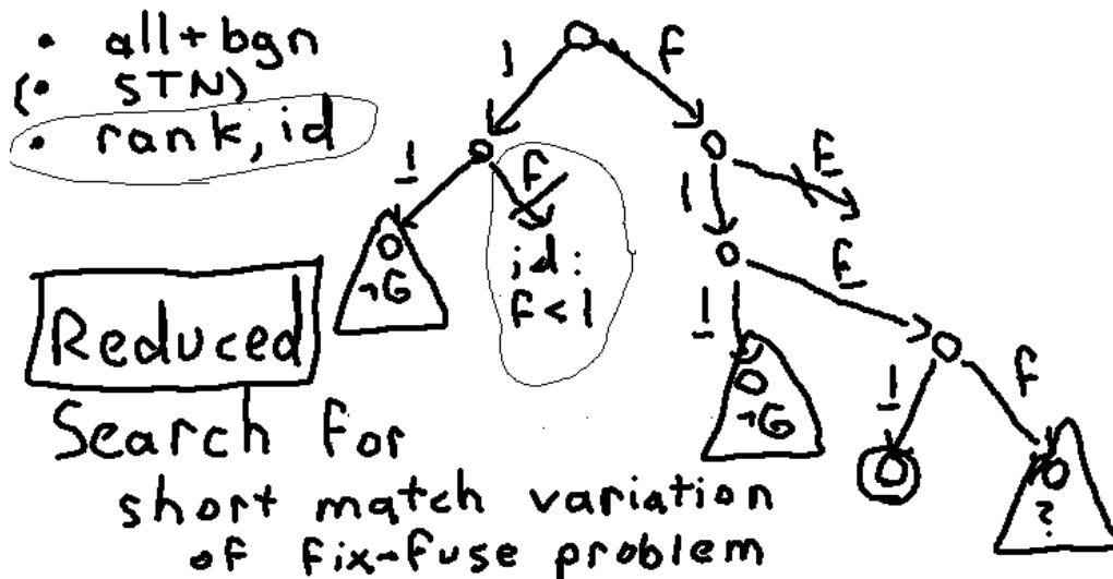
Figure 5.3: A deordered-slackless-reduced TEMPO search tree (cf. Theorem 5.16). Also see Section 5.3.1 and Figure 5.2.
