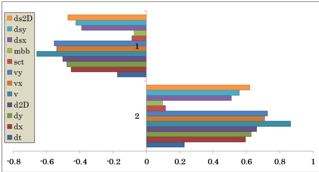
Figure 52. Cluster profile (TRACCLUS-MDL: k=2 ).
