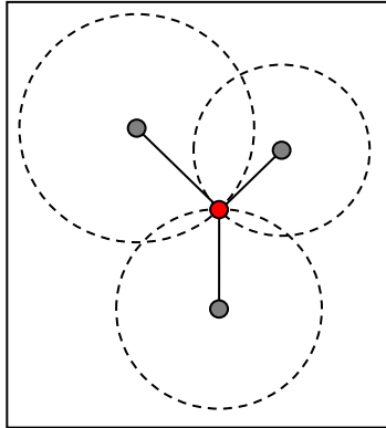
Figure 3. Trilateration technique to estimate two dimensional location. Adapted from Hightower & Borriello (2001).
