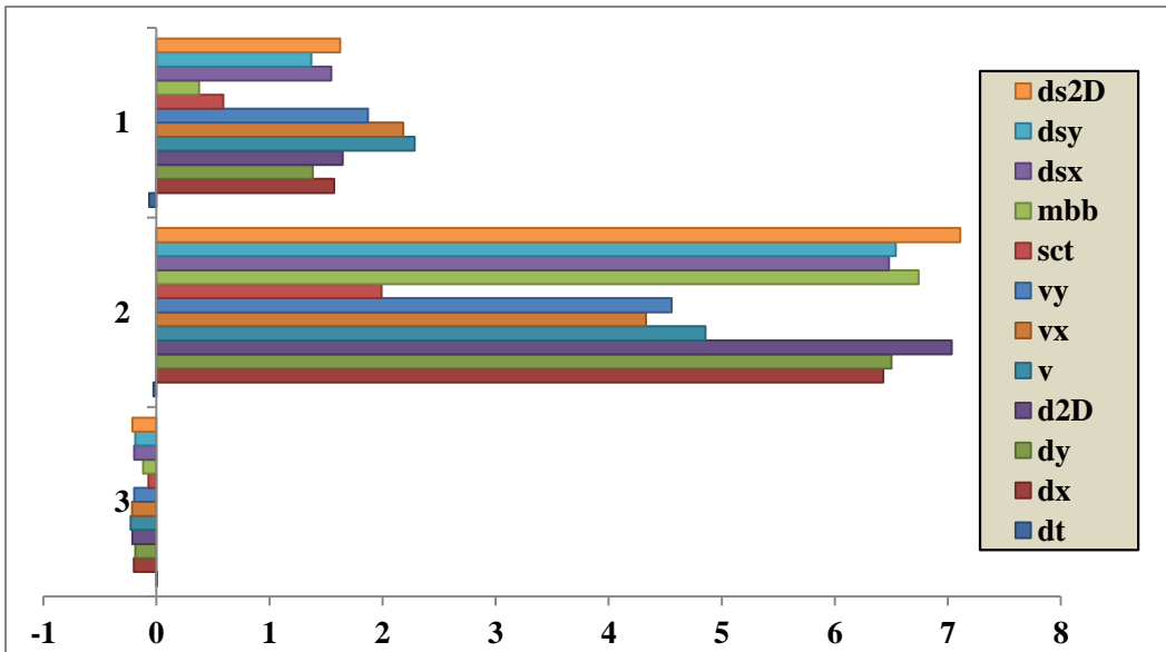
Figure 86. Cluster profile (TRACCLUS-MDL: k=3 ).
