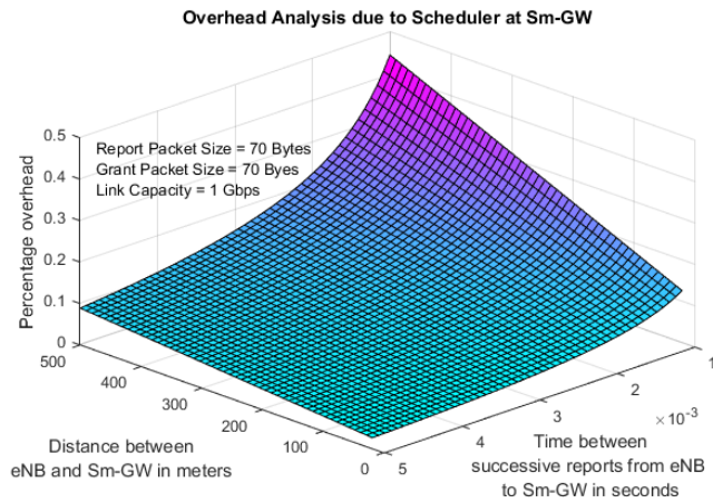
Figure 4.2: Overhead Analysis Due to Network Protocol Scheduler at the Sm-GW and Small Cell eNBs in the Indoor Environment ( 20m < d < 500m ).
