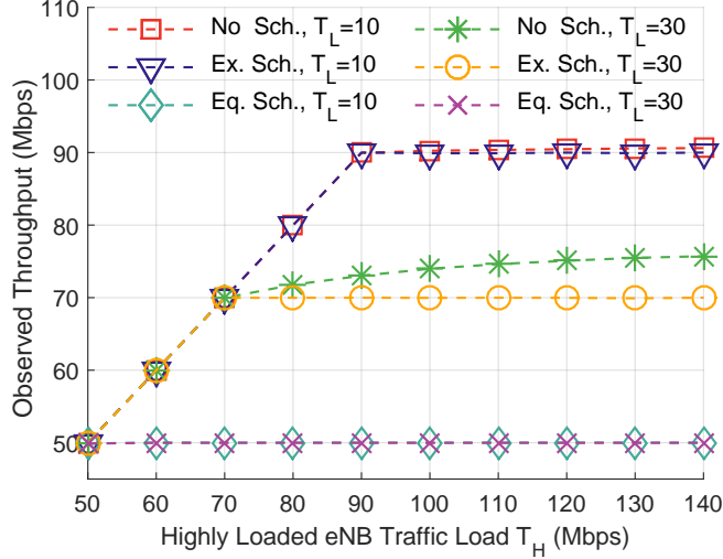
Figure 4.4: Observed Average Throughput of Highly Loaded eNBs.
