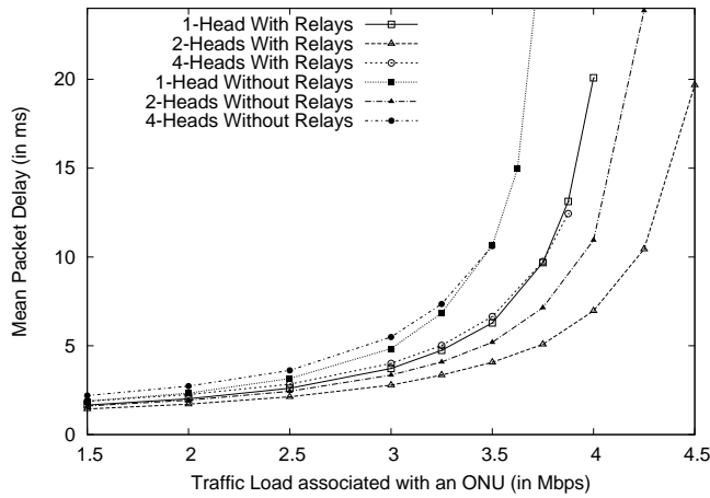
Figure 2.6: Clustered Routing With Relays: Mean Packet Delay As a Function of Traffic Load for Different Numbers of Cluster Heads in a Zone, With and Without Relays Between Adjacent Zones.
