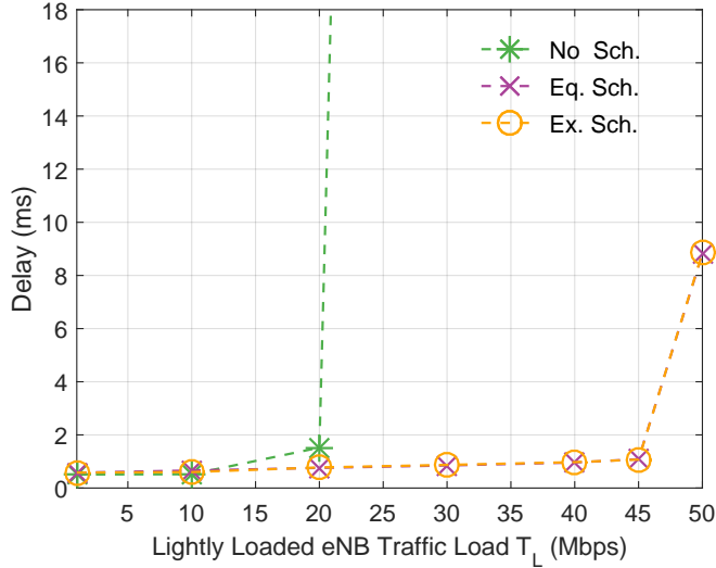
Figure 4.5: Average Delay of Lightly Loaded eNBs, When T_H = 80 Mbps.
