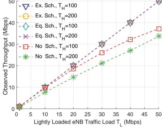
Figure 4.3: Observed Average Throughput of Lightly Loaded eNBs.
