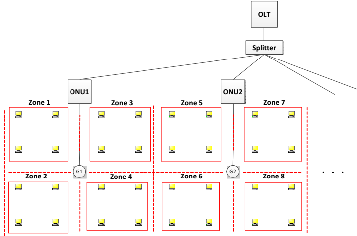
Figure 2.1: FiWi Network Structure: Wireless Nodes Are Organized Into Different Zones That Operate on Different Radio Frequencies (Channels).
