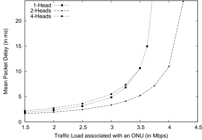
Figure 2.3: Clustered Routing: Mean End-to-End Packet Delay for Different Numbers of Cluster Heads in a Zone.
