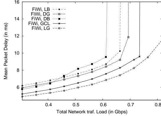
a) FiWi packet delay
