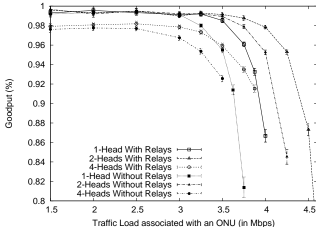
Figure 2.7: Clustered Routing With Relays: Normalized Goodput for Traffic With Delay Limit of 50 ms.
