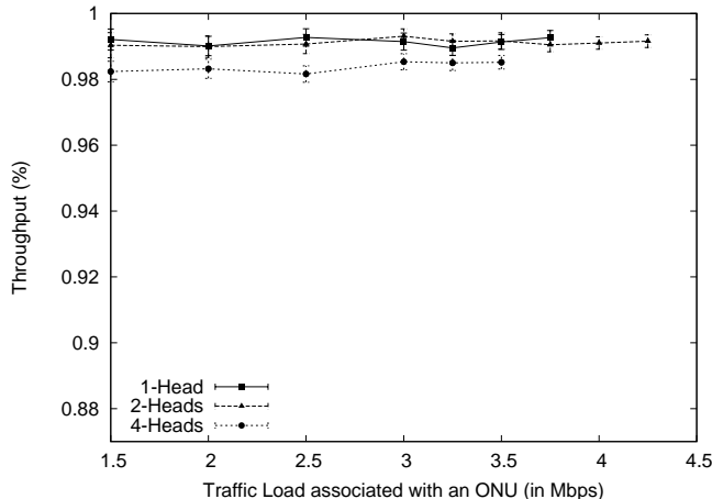
Figure 2.4: Clustered Routing: Normalized Throughput for Different Numbers of Heads.
