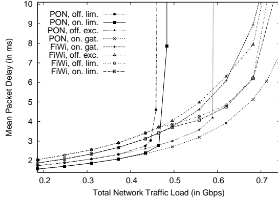
Figure 3.5: Mean Wireless (FiWi) and PON Packet Delays for Different DBA Mechanisms for CH-Server; STN-P2P Traffic. Fixed Parameters: 15–20 Km PON With Dedicated ONU Architecture, Cycle Length Z = 2 ms.
