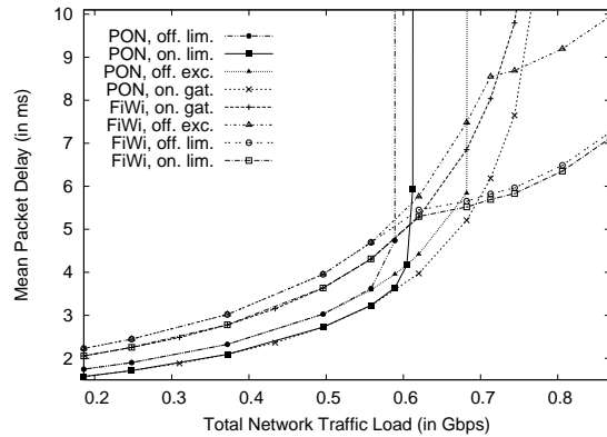
c) Cycle length Z = 4 ms
