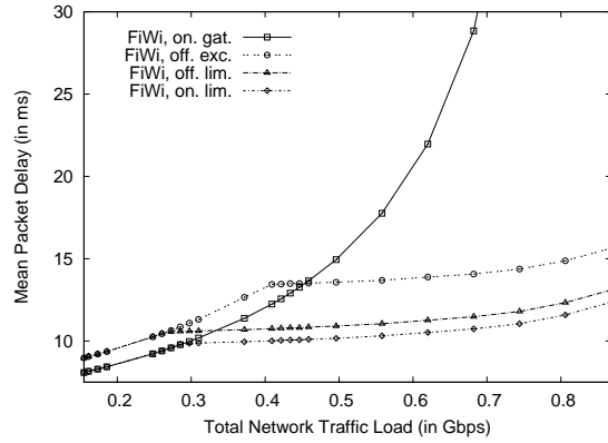
b) Cycle length Z = 4 ms
