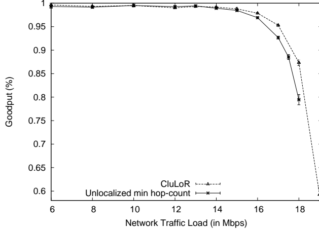
Figure 2.10: Localized Routing: Normalized Goodput for 50 ms Delay Limit for CluLoR Vs. Unlocalized Minimum Hop-Count Routing.
