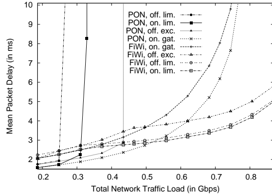
a) Cycle length Z = 1 ms
