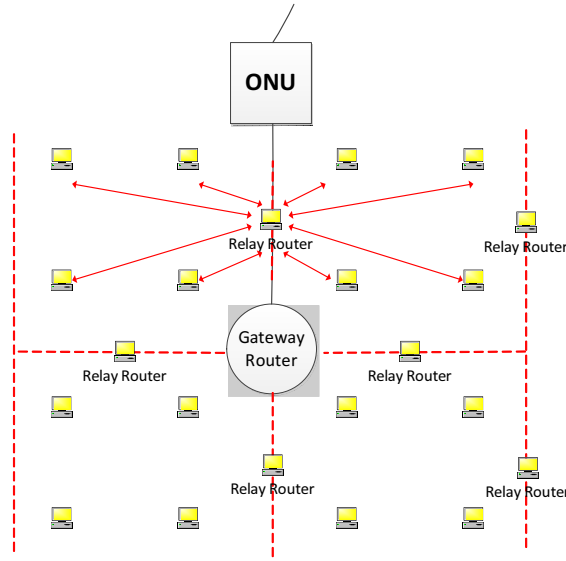
Figure 2.5: FiWi Network Structure With Relays Operating at the Two Radio Frequencies of the Two Adjacent Zones. Packets Destined to an Adjacent Zone Are Routed Through the Relay Router, Bypassing the Cluster Heads and Gateway Router.
