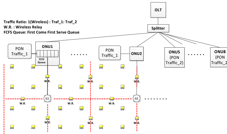
Figure 3.3: Mixed ONU FiWi Network Architecture Set-up: Four ONUs (ONUs 1–4) Serve a Mix of Wireless (FiWi) and Wired (PON) Traffic, While Four ONUs (ONUs 5–8) Serve Only Wired (PON) Traffic.
