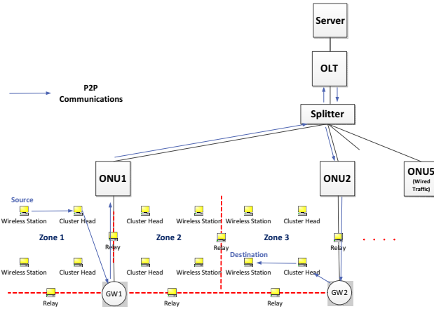
Figure 3.2: Dedicated ONU FiWi Network Architecture Set-up: Four ONUs (ONUs 1–4) Are Dedicated to Wireless (FiWi) Traffic While Four ONUs (ONUs 5–8) Are Dedicated to Wired (PON) Traffic. The Figure Also Illustrates CluLoR Routing: The Wireless Network Is Organized Into Zones, Each Operating at a Different Frequency. Wireless Stations Route Traffic Through a Cluster Head Towards the Gateway for Transmission Over the PON.
