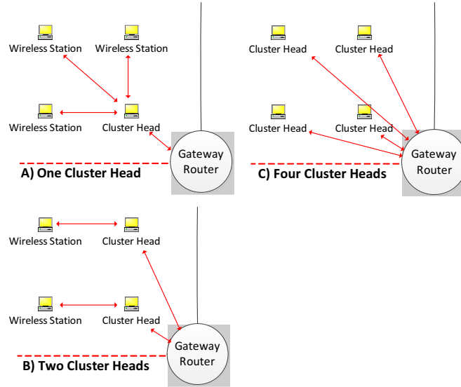
Figure 2.2: Illustration of Clustered Routing With Different Numbers of Cluster Heads in a Zone: Wireless Nodes Direct All Communication With Nodes Outside the Zone Through a Cluster Head. The Cluster Communicates With the Gateway Router, Which Is Connected to an ONU. The Configuration With 4 Heads Corresponds Effectively to an Unclustered Benchmark As All Nodes Communicate Directly (Without Going Through a Cluster Head) With the Gateway Router.
