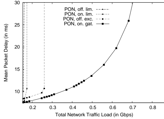
a) Cycle length Z = 2 ms
