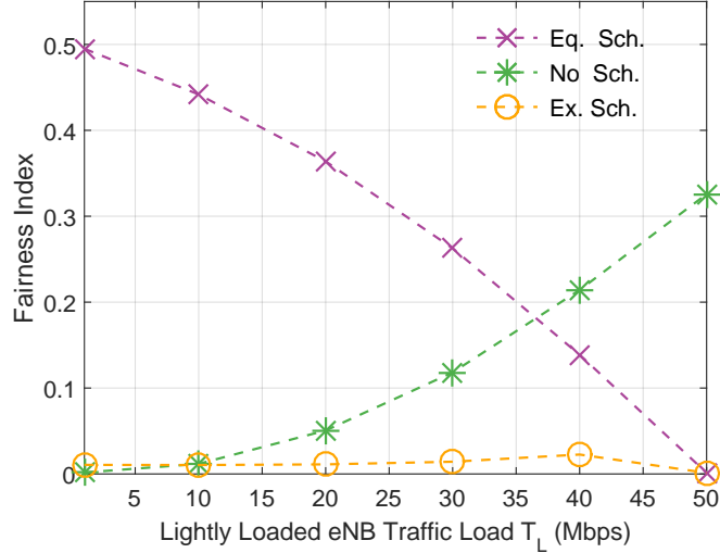
Figure 4.6: Fairness Index \mathcal{F}_T , When T_H = 200 Mbps.
