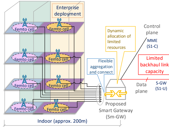
Figure 1.1: Enterprise Deployment of Small (Femto) Cells: The Proposed Smart Gateway (Sm-GW) Is Inserted Between the Femto Cell Base Stations (LTE eNBs and Access Points) and the Conventional Backhaul Entities, Such As LTE MME and S-GW. The Sm-GW Flexibly Connects to a Multitude of Femto Cell Base Stations and Dynamically Allocates the Limited Backhaul Capacity to the Different Femto Cells.
