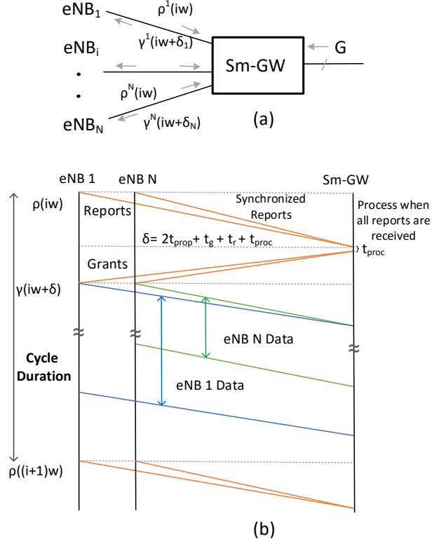
Figure 4.1: Illustration of Smart Gateway (Sm-GW) Function: (a) Sm-GW Receives Backhaul Transmission Bitrate Allocation G From Operator. Based on Uplink Transmission Bitrate Requests (Reports) \rho_n From Individual eNBs n, 1, \dots, N , Sm-GW Gives Uplink Transmission Grants \gamma_n to the eNBs. \delta Represents the Granting Delay. (b) The eNB Requests (Reports) \rho_n and Sm-GW Grants \gamma_n Are Followed by the eNB Uplink Data Transmissions (in Parallel) in a Fixed-Period Cycle.
