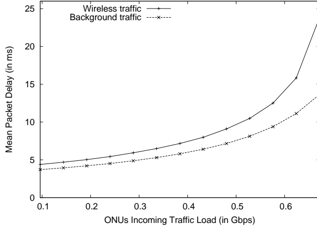
Figure 2.11: Mean End-to-End Packet Delay for PON With Fiber Background Traffic (32 ONUs With 2:1 Ratio of Background Traffic : Peer-to-Peer Wireless Station Traffic).
