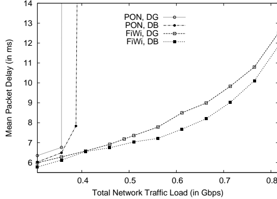
Figure 3.11: Mean FiWi and PON Packet Delays for Distance Grouping (DG) and Distance Balancing (DB) ONU Grouping Strategies for (dpp., lim.) DBA Mechanism. Fixed parameters: Mixed ONU Architecture With 80–120 Km Long-Range Propagation, Z = 4 ms Cycle Length, All-P2P Traffic With Ratio 1:10:40.
