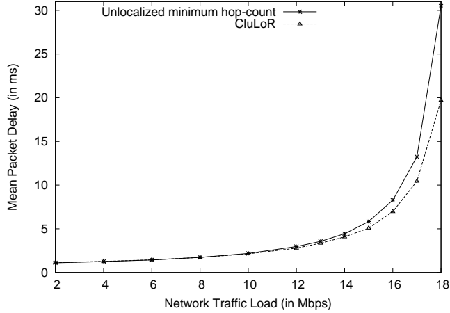
Figure 2.9: Localized Routing: Mean Packet Delay for CluLoR Vs. Unlocalized Minimum Hop-Count Routing.
