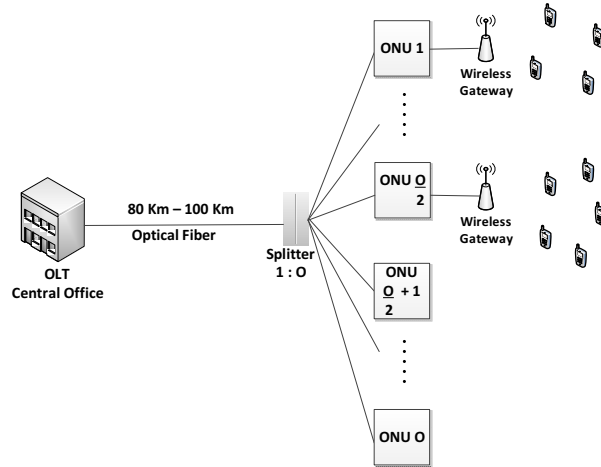
Figure 3.1: Illustration of Long-Reach (LR) FiWi Network Architecture: Distributed Optical Network Units (ONUs) Are Connected Via Optical Fiber to a Central Optical Line Terminal (OLT). Some of the ONUs Support Via Wireless Gateways the Communication of Distributed Wireless Stations.
