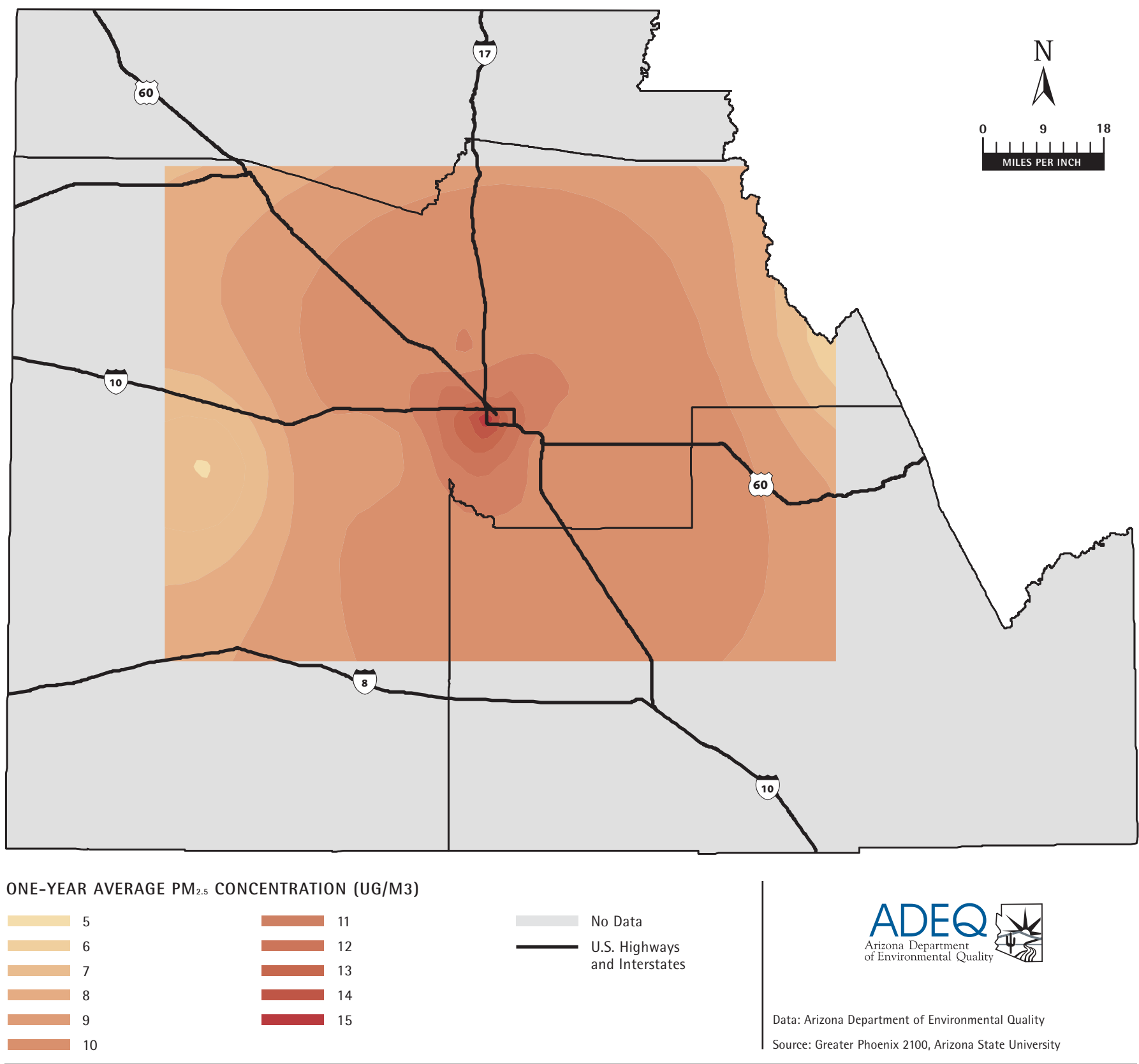
Map 17: One-Year Average Concentrations of Fine (PM 2.5 ) Particulates, 2000
