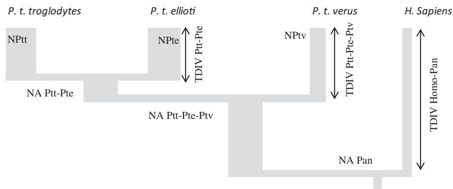
Fig. 2. —Schematic representation of the inferred demographic history of the three subspecies: Pan troglodytes troglodytes (Pt t ); P. t. verus (Ptv); and P. t. ellioti (Pte). NA, ancestral effective population size; N, effective population size; TDIV, divergence time.
