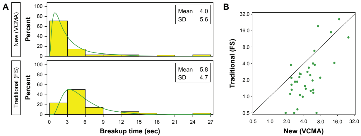
Figure 4 Tear film breakup time observations for new (VCMA) and traditional (FS) methods for 17 dry-eye subjects (34 eyes). (A) Observed (yellow) and modeled (green, lognormal) histogram. (B) Scatter plot of the new versus traditional observations relative to a 45° reference line. Sample means were 4.0 for VCMA and 5.8 for FS. Abbreviations: FS, forced-stare; SD, standard deviation; VCMA, video capture manual analysis.
