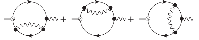
FIG. 1. The leading radiative corrections to the axial current in the linear in magnetic field approximation. Solid and wavy lines correspond to the fermion and photon propagators, respectively. Double solid lines describe the axial current insertions and the external wavy lines attached to the fermion loops indicate the insertions of the external gauge field.
