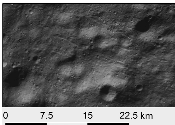
Fig. 14. Type area of the grooves, which is located at 23°N, 117°E. There are many closely spaced grooves in this area.
