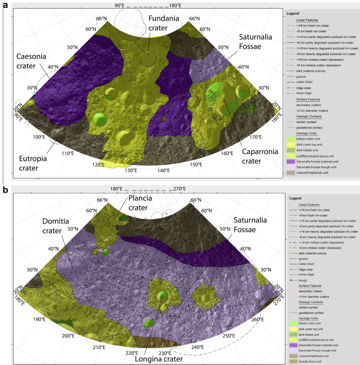
Fig. 6. (a) Geological map of Caparronia quadrangle. This map contains all of the mapped features, including craters <6 km in diameter. Description of the mapped units and structural features is included in Section 4. A high resolution version is available in the Supplementary material . (b) Geological map of Domitia quadrangle. This map contains all of the mapped features, including craters <6 km in diameter. Description of the mapped units and structural features is included in Section 4. A high resolution version is available in the Supplementary material .
