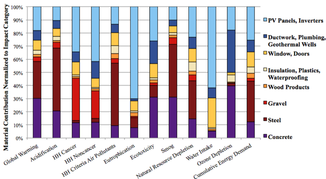
Figure 3. Life cycle environmental impacts of building materials by material type for net-zero energy building (PV = photovoltaic).
