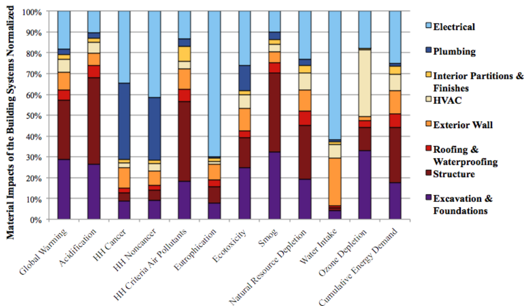
Figure 3. Life cycle environmental impacts of building materials by material type for net-zero energy building (PV = photovoltaic).
