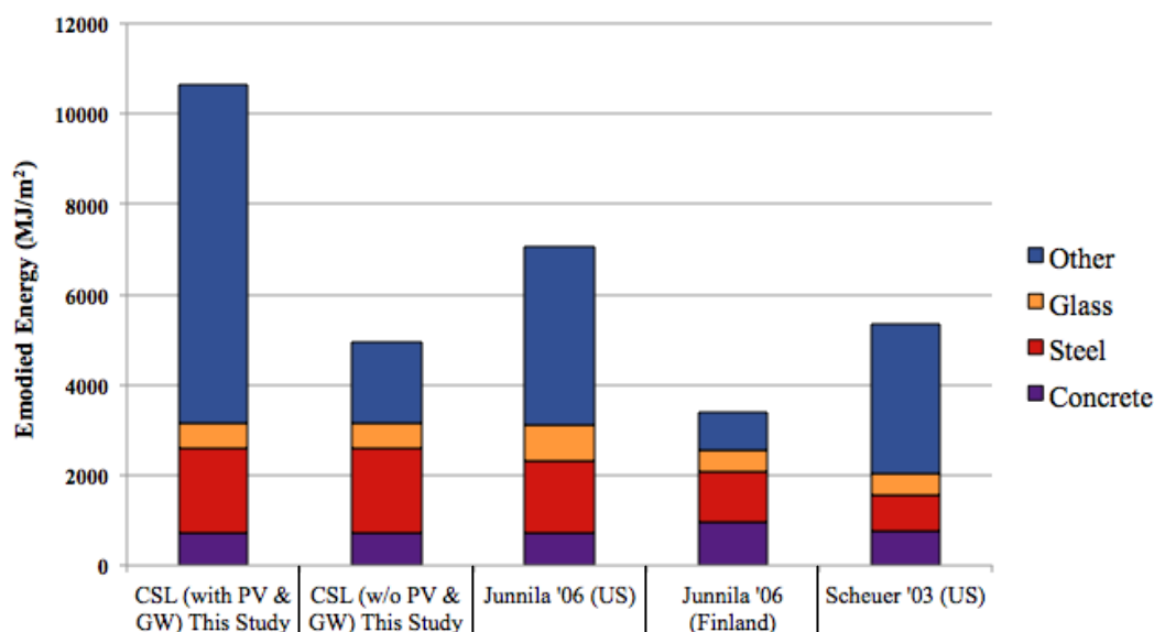
Figure 5. Embodied energy comparison between the Net-Zero Energy CSL building and published LCA building studies; PV = Photovoltaic & Inverters; GW = Geothermal Wells; Note: Junnila '03 and Kofoworola '07 did not report on embodied energy.
