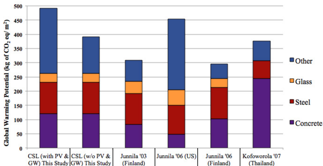
Figure 4. Global warming potential of the CSL compared to the published results. PV = Photovoltaic & Inverters; GW = Geothermal Wells; Note: The Kofoworola '07 study did not report glass separately from other materials; it is therefore represented in the “other” category.
