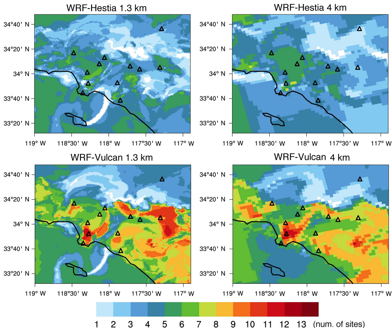
Figure 14. Composite maps of spatial correlation ( R in Figs. 12 and 13) for the 1.3 km WRF-Hestia, 1.3 km WRF-Vulcan, 4 km WRF-Hestia, and 4 km WRF-Vulcan runs. Each composite map was constructed by determining the number of the observation sites for which |R| is greater than 0.46 at each grid cell. |R| = 0.46 is the critical value at the significance level of 0.01 of t test. Specifically, white cells indicate that no sites are correlated well at the location; dark red cells indicate that over 13 sites have good correlation at the location. The SCI and Dryden sites are not shown on these maps.
