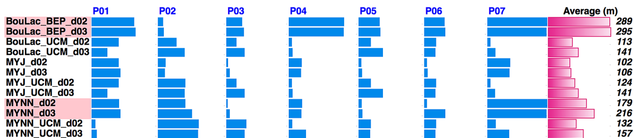
Figure 3. Absolute difference between the aircraft-determined and modelled PBL height for each profile: P01–P07 (blue bars). The pink bars in the last column represent the averaged bias over all of the profiles for each configuration. Note that the shorter the bar, the better agreement of the model with the observations.
