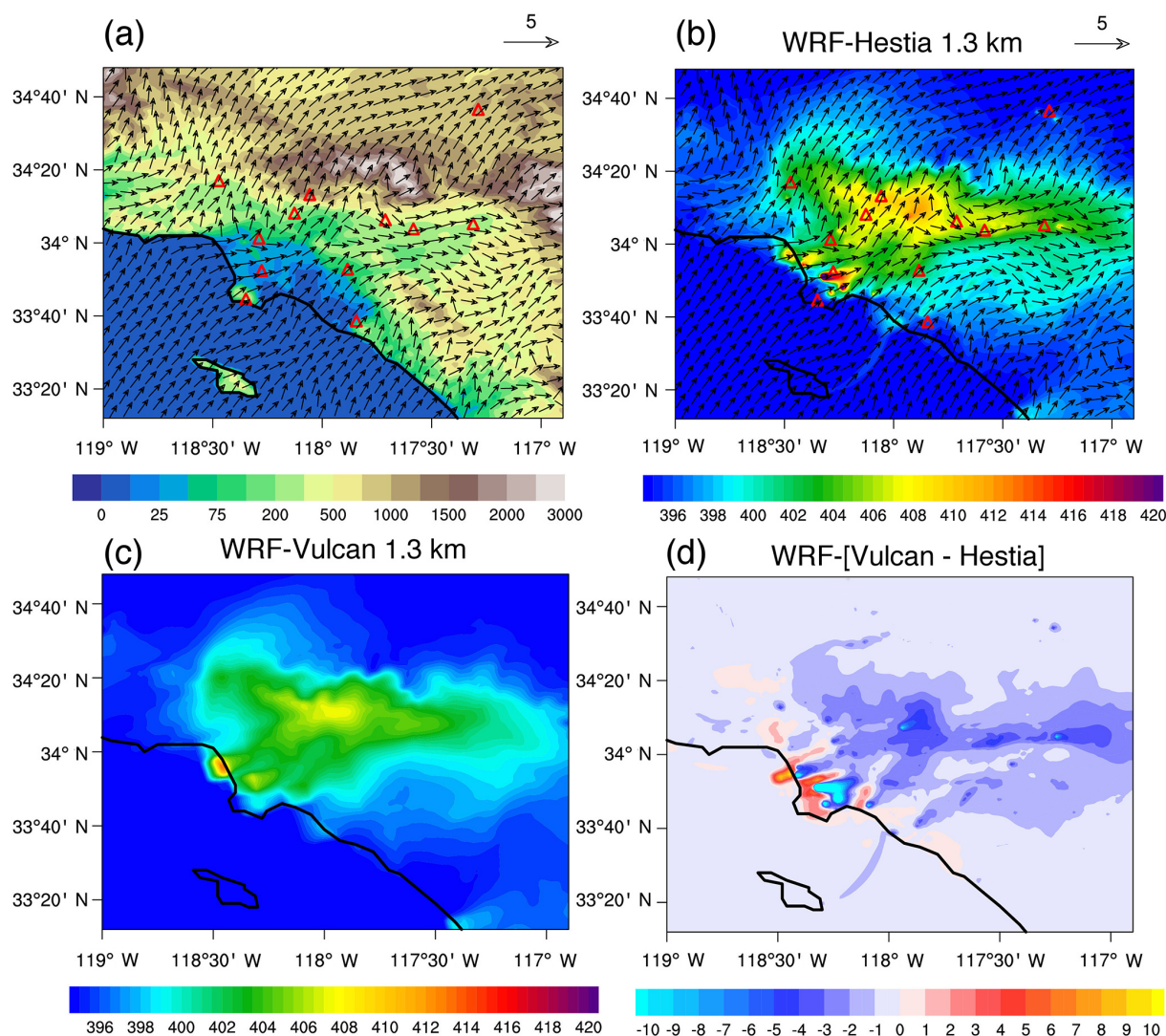
Figure 11. (a, b) The first empirical orthogonal function (EOF 1) for the surface wind pattern (black arrows) simulated by MYNN_UCM_d03 at 14:00 PST during CalNex-LA. EOF 1 accounts for 48.1% of the variance in the average winds. Contours: (a) terrain height (unit: m); (b) the modelled surface CO 2 concentration (unit: ppm) from the 1.3 km WRF-Hestia run. The red triangles indicate the locations of the GHG measurement sites. (c) The modelled CO 2 concentrations from the 1.3 km WRF-Vulcan run (unit: ppm). (d) The difference in the modelled CO 2 concentrations between the 1.3 km WRF-Vulcan and WRF-Hestia runs (unit: ppm).
