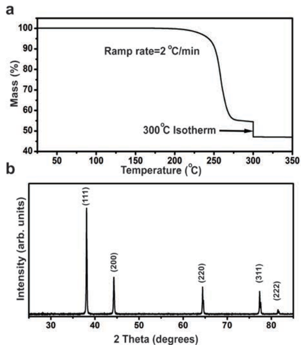
Figure 2. (a) Thermogravimetric analysis on silver benzoate. The temperature ramp rate was 2°C/min and a 2 hr isotherm was applied at 300°C. (b) X-ray diffraction pattern of silver made via the thermal decomposition of silver benzoate.
