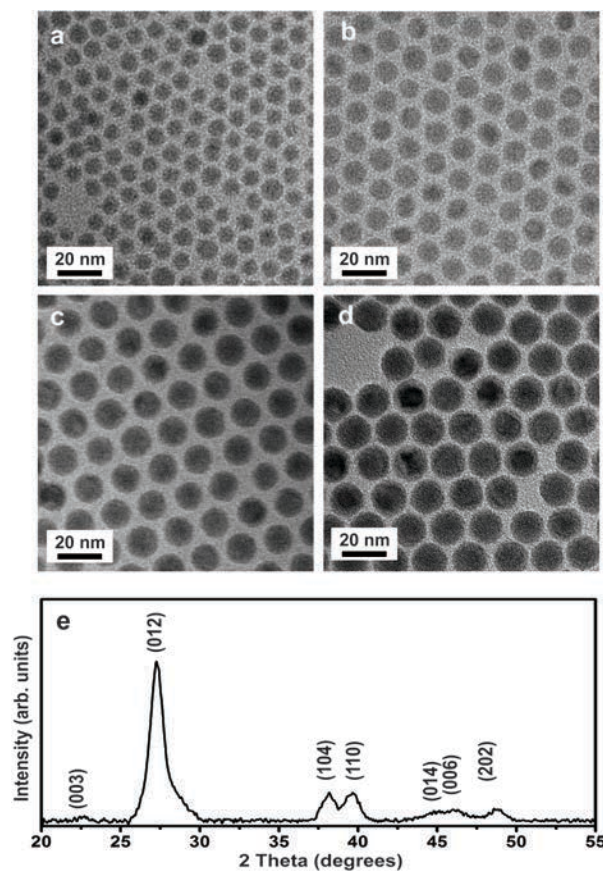
Figure 1. Transmission electron microscopy images of the Bi nanoparticles used to create the Ag matrix – Bi nanoparticle composites. The nanoparticle diameters are (a) 8.1 \pm 1.0 nm, (b) 9.8 \pm 0.8 nm, (c) 13.2 \pm 0.6 nm and (d) 14.9 \pm 0.6 nm. (e) X-ray diffraction pattern of Bi nanoparticles with 13.6 nm diameter.
