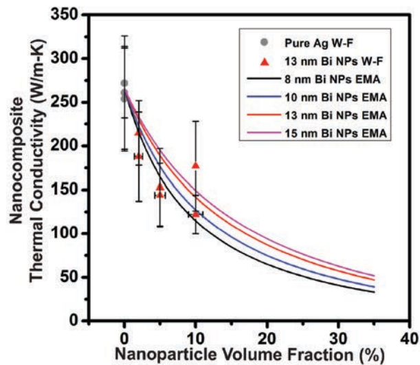
Figure 6. Nanocomposite thermal conductivity measurements using the Wiedemann-Franz (W-F) law and thermal conductivity calculations using the modified effective medium approximation (EMA) for varying nanoparticle (NP) diameter and volume fraction.
