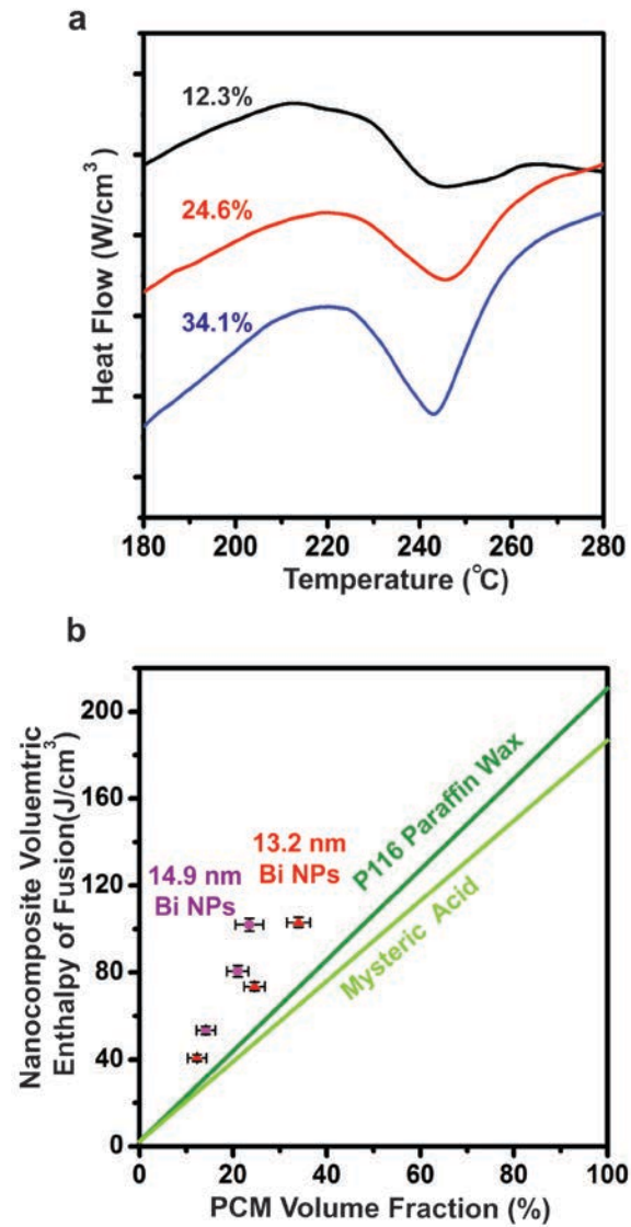
Figure 5. (a) The endothermic melting valley during DSC measurements on composites with 13.2 nm diameter Bi nanoparticles and varying Bi volume fraction. For clarity, the data in part
