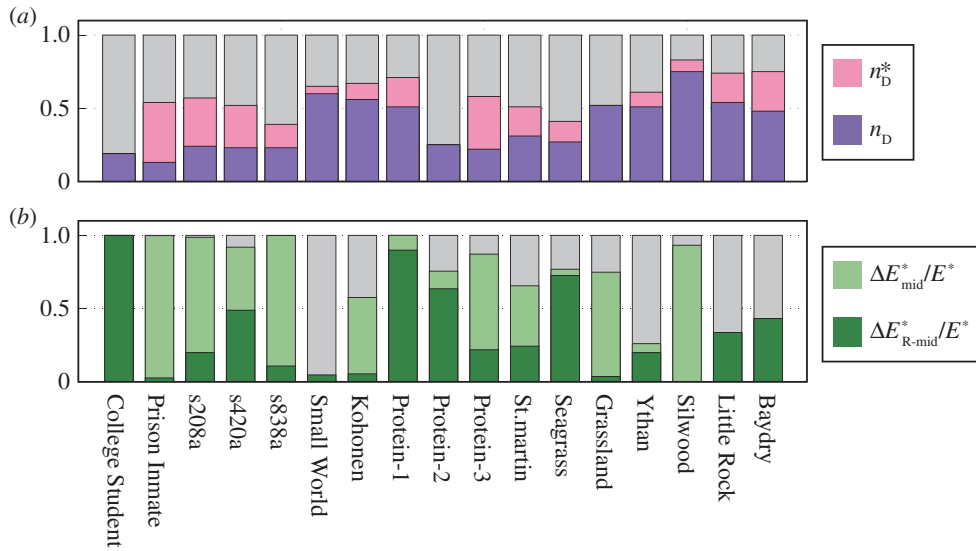
Figure 4. For the 17 real-world networks studied in [10], (a) densities of the original driver nodes n_D (dark purple) and of the augmented controls n_D^* (light purple). (b) Normalized energy reduction \Delta E_{\text{mid}}^*/E^* = (E^* - E_{\text{mid}}^*)/E^* (light green) when an additional control signal is added to the middle of each LCC and normalized energy reduction \Delta E_{\text{R-mid}}^*/E^* = (E^* - E_{\text{R-mid}}^*)/E^* (dark green) for the case where the same number of control signals are randomly added into each network. All coloured bars start from 0. For the ‘Silwood’ network, the energy with randomly added control signals is higher than the corresponding E^* (the negative \Delta E_{\text{R-mid}}^* is not shown in the figure). For the light green bars, the reduced control energy E_{\text{mid}}^* is several orders of magnitude smaller than E^* . The bars with more gray portion than the light green portions are for the networks with relatively low values of E^* and D_C , for which energy reduction is not necessary.
