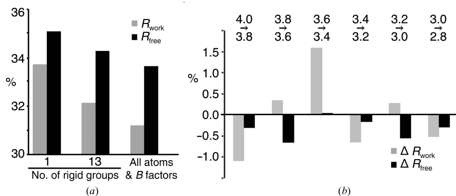
Figure 2 R work and R free values resulting from different refinement strategies. (a) R values after refinement with increasing numbers of parameters, including data to 4.0 Å resolution. (b) Differences in R values after refinement (all atom coordinates, individual B factors) depending on the chosen high-resolution data cutoff. Models were refined in parallel to both the lower and the higher resolution cutoff and the R values were compared at the lower cutoff. The range of lower data quality between 3.6 and 3.4 Å is probably caused by high background scattering owing to the solvent.
