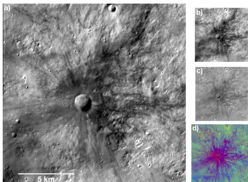
Fig. 10. Dawn FC images of a small dark-rayed impact crater Laeta, west of crater Marcia, located at 14^\circ\text{N} , 180^\circ . (a) LAMO image, spatial resolution 25 m/pixel; (b) HAMO image, spatial resolution 70 m/pixel; (c) photometrically-corrected HAMO image, spatial resolution 70 m/pixel; (d) HAMO Clementine-type color ratio image, spatial resolution 70 m/pixel. This dark-rayed crater may be excavating part of a subsurface regional dark layer, as exposed in the SW wall of Marcia (Fig. 11). (For interpretation of the references to colour in this figure legend, the reader is referred to the web version of this article.)
