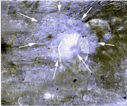
Fig. 9. Dawn FC image mosaic showing the spectral signature of a potential earlier impact (outlined by white arrows) centered near the northwestern rim of Marcia. This sharp eccentric boundary is without counterpart in the DTM, which would be unexpected for an ejecta sheet from Marcia, and in fact does not coincide with that respective unit. The different spectral properties can be explained as a result of a major earlier impact that replaced the surface material with a mixture of deeper layers. Then the later Marcia impact and its ejecta erased most the topographic signature of the earlier event. In the northwestern part of Marcia, near the center of the old impact, the change of the composition is more prominent because of the more distinct combination of the excavated material. Red and Green channels: 440 \text{ nm}^3 / (650 \text{ nm} * 750 \text{ nm} * 830 \text{ nm}) , Blue channel: 960 \text{ nm} / 830 \text{ nm} . (For interpretation of the references to colour in this figure legend, the reader is referred to the web version of this article.)
