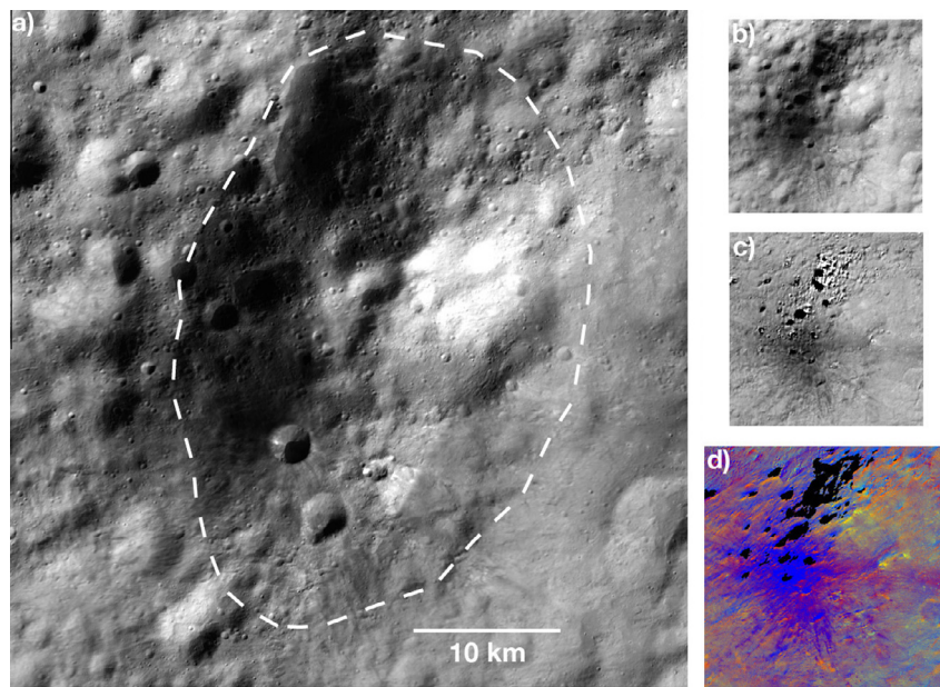
Fig. 15. Dawn FC mosaics of Aricia Tholus, located at 12^{\circ}\text{N} , 162^{\circ}\text{E} . Dashed white line marks the boundary of the topographic high as seen in the DTM. (a) LAMO image, spatial resolution 25 m/pixel; (b) HAMO image, spatial resolution 70 m/pixel; (c) photometrically corrected HAMO image, spatial resolution 70 m/pixel, enables separation of shadows from truly dark material; (d) HAMO Clementine-type color ratio image, spatial resolution 70 m/pixel. (For interpretation of the references to colour in this figure legend, the reader is referred to the web version of this article.)
