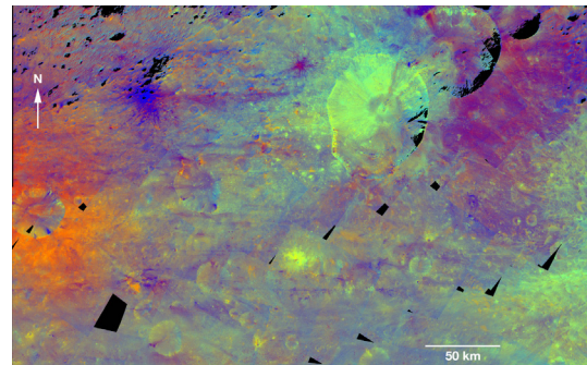
Fig. 3. FC HAMO-derived Clementine-type color ratio mosaic of Av-8 Marcia quadrangle. Spatial resolution is 70 m/pixel. Colors correspond to Red: 750/430 nm, Green: 750/920 nm, and Blue 430/750 nm. Mosaic is Mercator projection, centered on longitude 180° (Claudia coordinate system: Russell et al., 2012; Roatsch et al., 2012).
