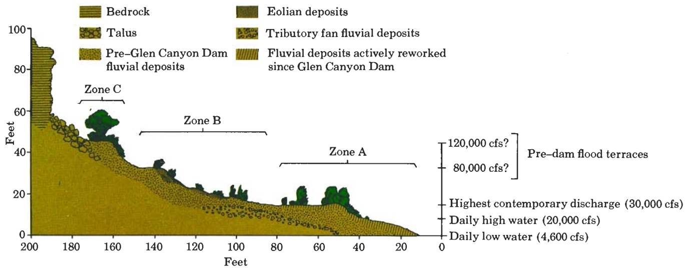
Figure 4. The cross section shows an idealized river deposit under post-dam conditions. The characteristics of the vegetation, sediments, and human use of the 3 zones are listed in Table 2.
