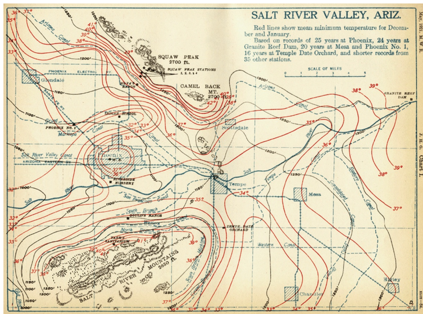
FIG. 3. Mean winter (Dec and Jan) minimum temperatures ( ^{\circ}\text{F} ) during the early twentieth century for the Salt River Valley, which includes a notable elevated isotherm pattern over the City of Phoenix (Source: Gordon 1921).
