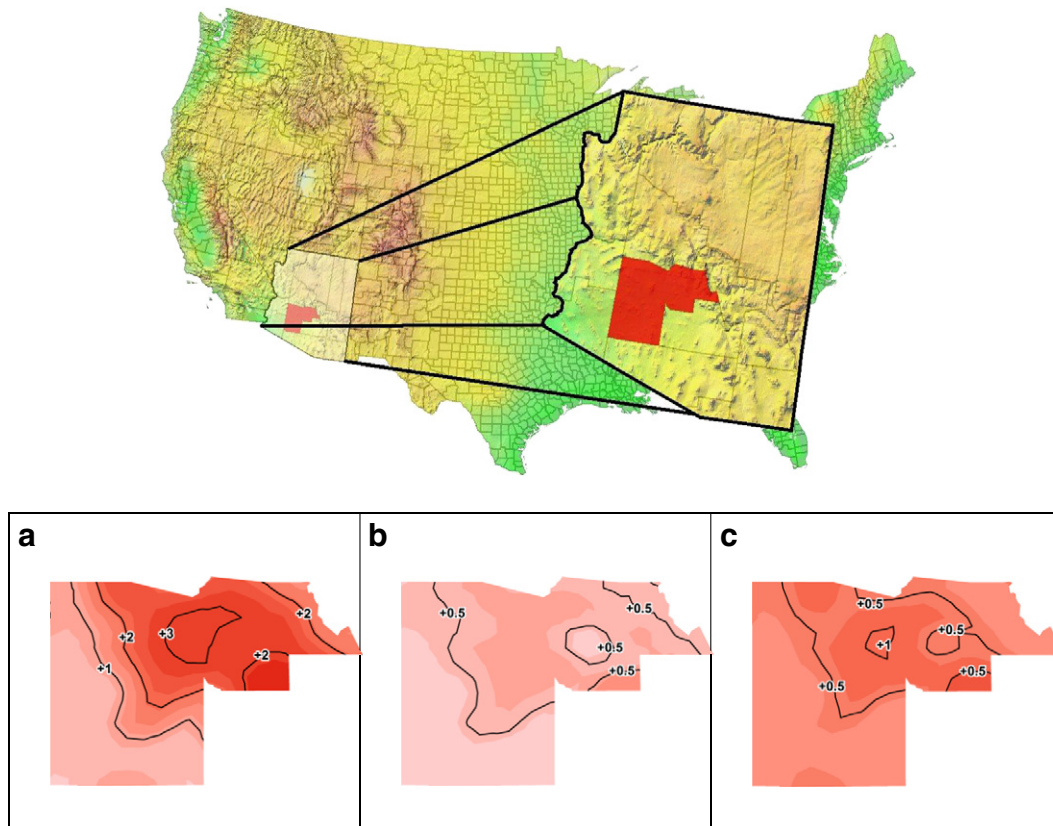
Fig. 1. A map highlighting the study region, Maricopa County, Arizona, United States. The insets show projected changes in summer mean daily temperatures ( ^{\circ}\text{C} ) in Maricopa County under (a) a high-growth scenario (SunCorrHi), (b) a low-growth scenario (SunCorrLow), and (c) an adaptation scenario (SunCorrAdapt) for year 2050.
