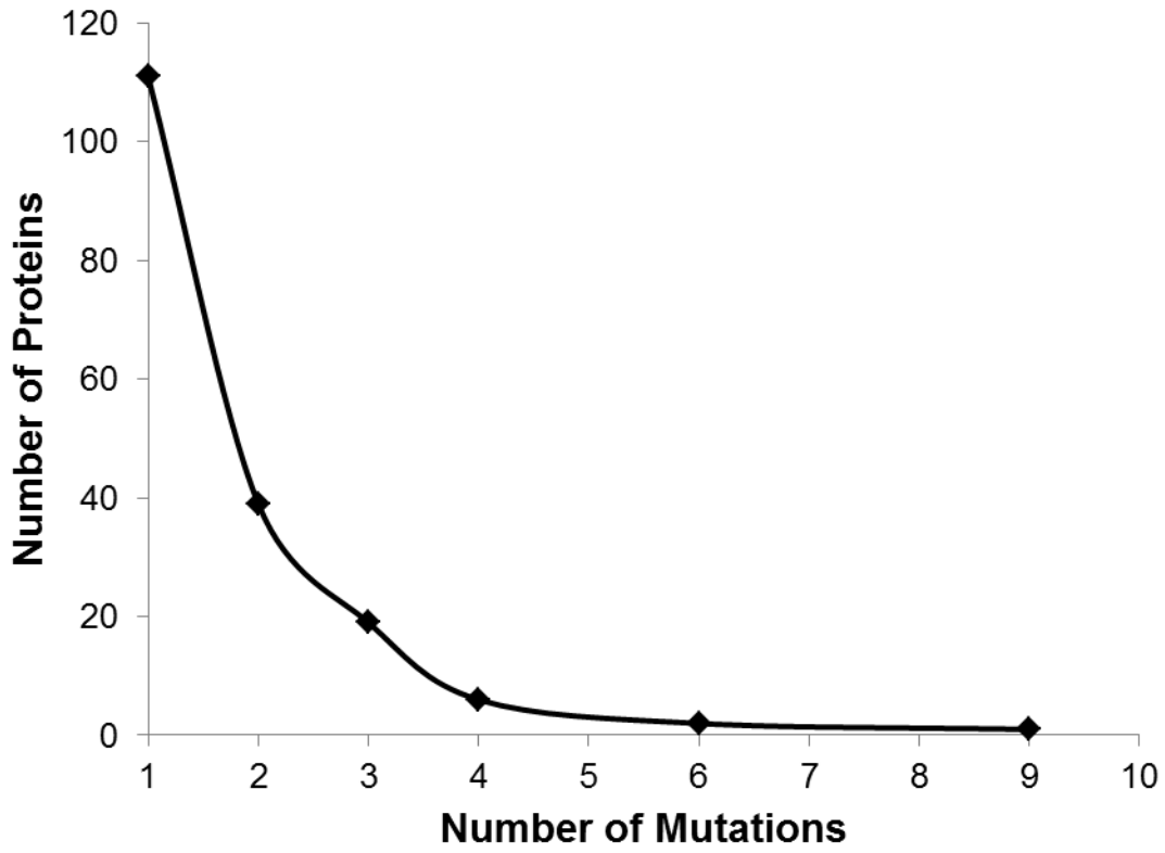
Figure S1. The distribution of the nsSNVs across different family of proteins. (Data can be found in “SuppTableforFigureS1.xlsx”)
