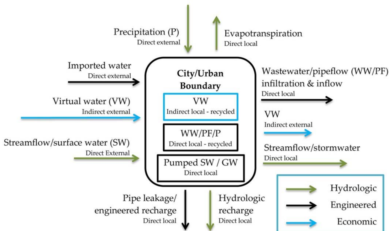
Figure 1. Conceptual diagram of the direct and indirect water flows of an urban area. The recycling of direct and indirect local water within the urban boundary is also identified. Flows are defined as local and external if they originate from within or outside the urban boundary, respectively. Flows are also identified as hydrologic, engineered, and economic.
