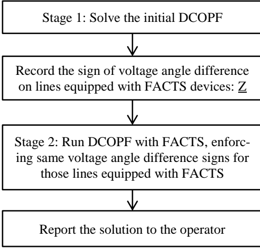
Fig. 1. The two-stage LP-based algorithm for enhanced operation of FACTS devices.
